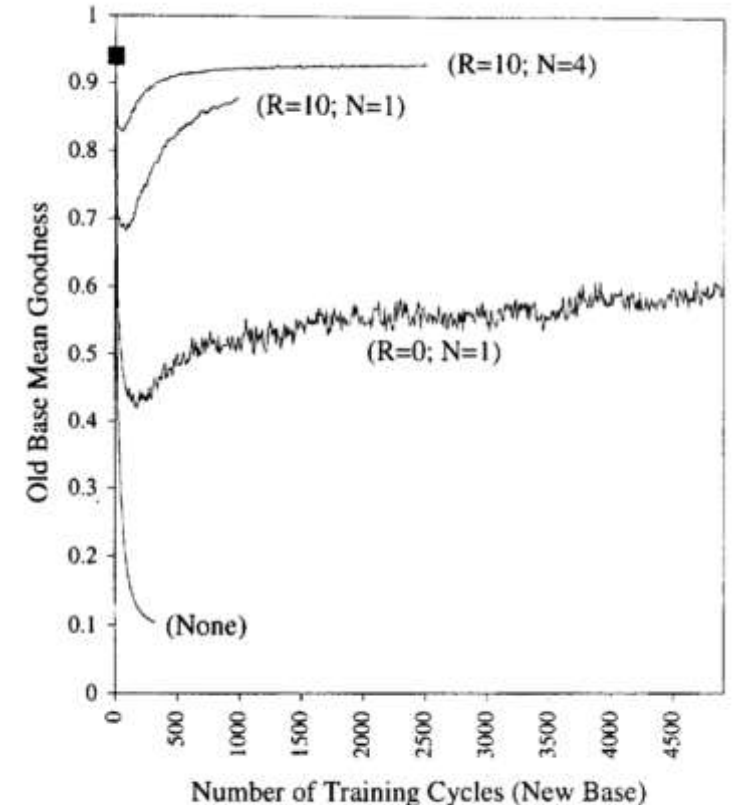
Figure 5. Mean goodness of the old base as a function of the number of training cycles of the new base.
